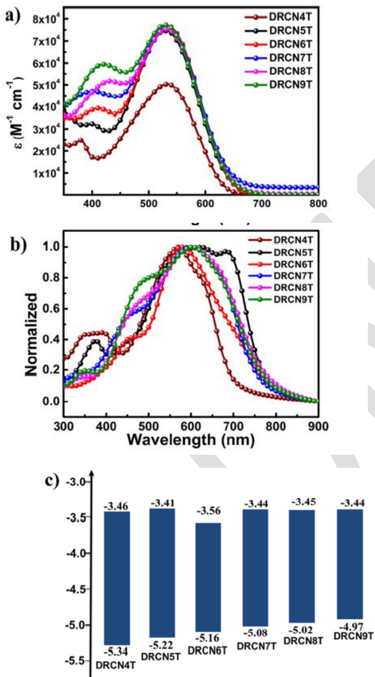
(a) UV-vis absorption spectra of DRCN4T-DRCN9T solutions. (b) UV-vis absorption spectra of DRCN4T-DRCN9T films. (c) HOMO and LUMO energy levels of DRCN4T-DRCN9T.
