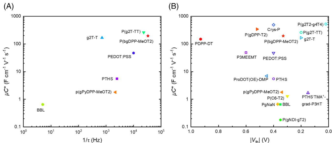
FIGURE 8 Summary of OECT performances via (A) \mu C^* - 1/\tau , and (B) \mu C^* - |V_{th}| plot for the polymers in Table 1. The polymers in the upper right corner of both images have better overall properties. The response speed is limited to 1– 10^5 Hz for OECTs and shows a large variation among polymers. Although the \mu C^* value of many polymers is outstanding, the |V_{th}| of the device is unsatisfactory, which is more obvious in D–A polymers. OECT, organic electrochemical transistor
