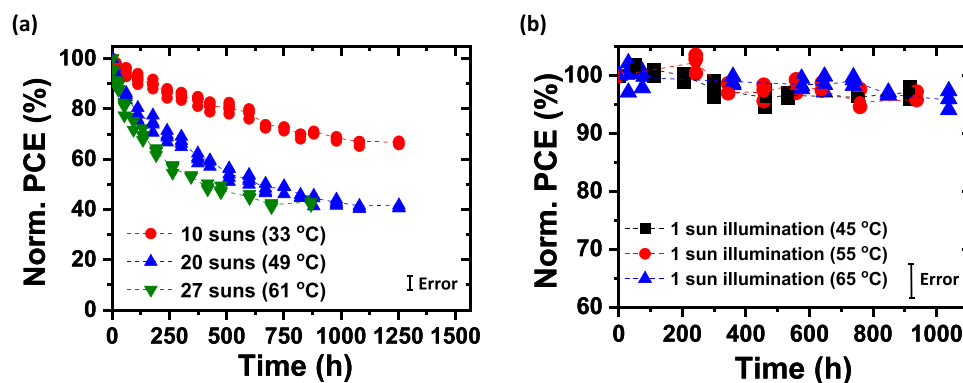
Fig. 2 OPV efficiency under accelerated aging conditions. a Normalized PCE plotted vs. aging time under illumination equivalent to 10 \pm 1.2 , 20 \pm 2.5 , and 27 \pm 3.8 suns. b Normalized PCE plotted vs. aging time under simulated AM1.5 G one sun illumination with temperature of 45 \pm 5 , 55 \pm 5 , and 65 \pm 5 °C (populations of 3–4 devices). The error bars indicate the 1 s.d. uncertainty of PCE measurements.
