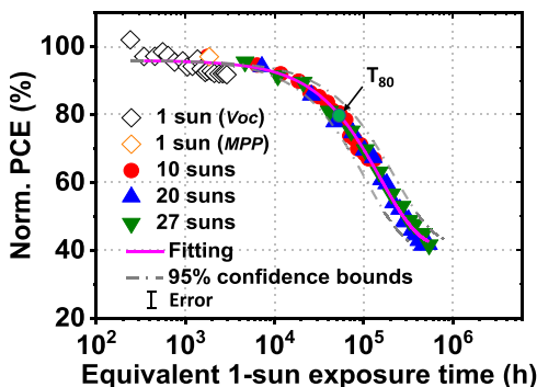
Fig. 6 Aging acceleration factor and extrapolated OPV lifetime.
